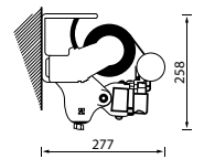
Australia R-90 Wall/Face Fix
